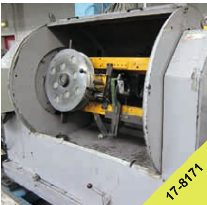
KLASREPOHL Dual excentric taping head
