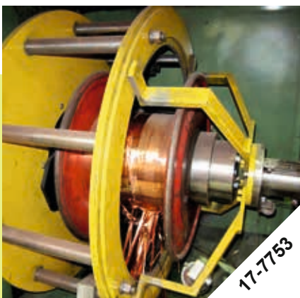
DUNST Concentric taping machine for copper tape, KBW 56
